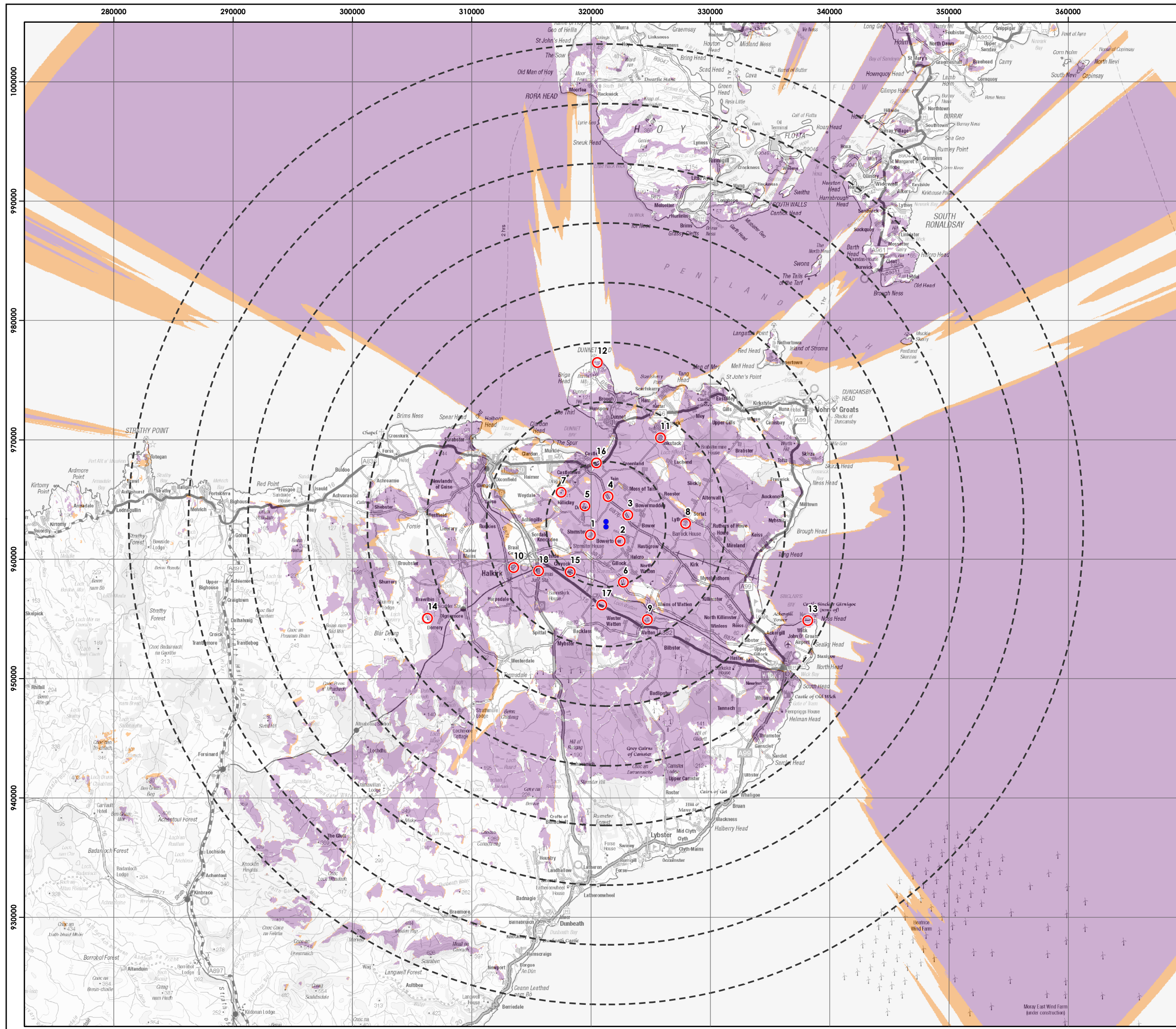
Figure 5-1-4a Blade Tip Zone of Theoretical Visibility
