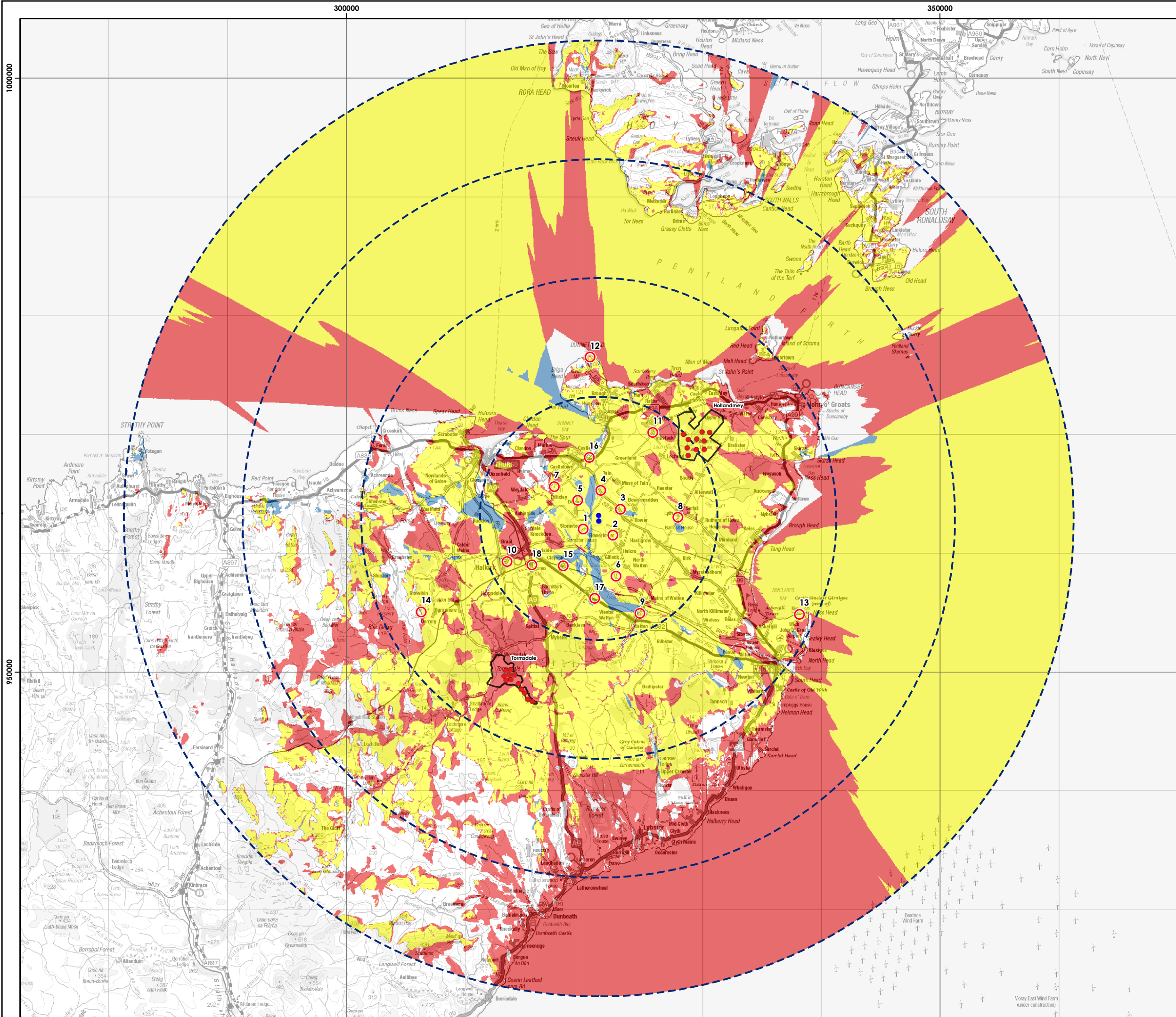
Figure 5-1-9b Cumulative Blade Tip ZTV: Hollandmey and Tormsdale
