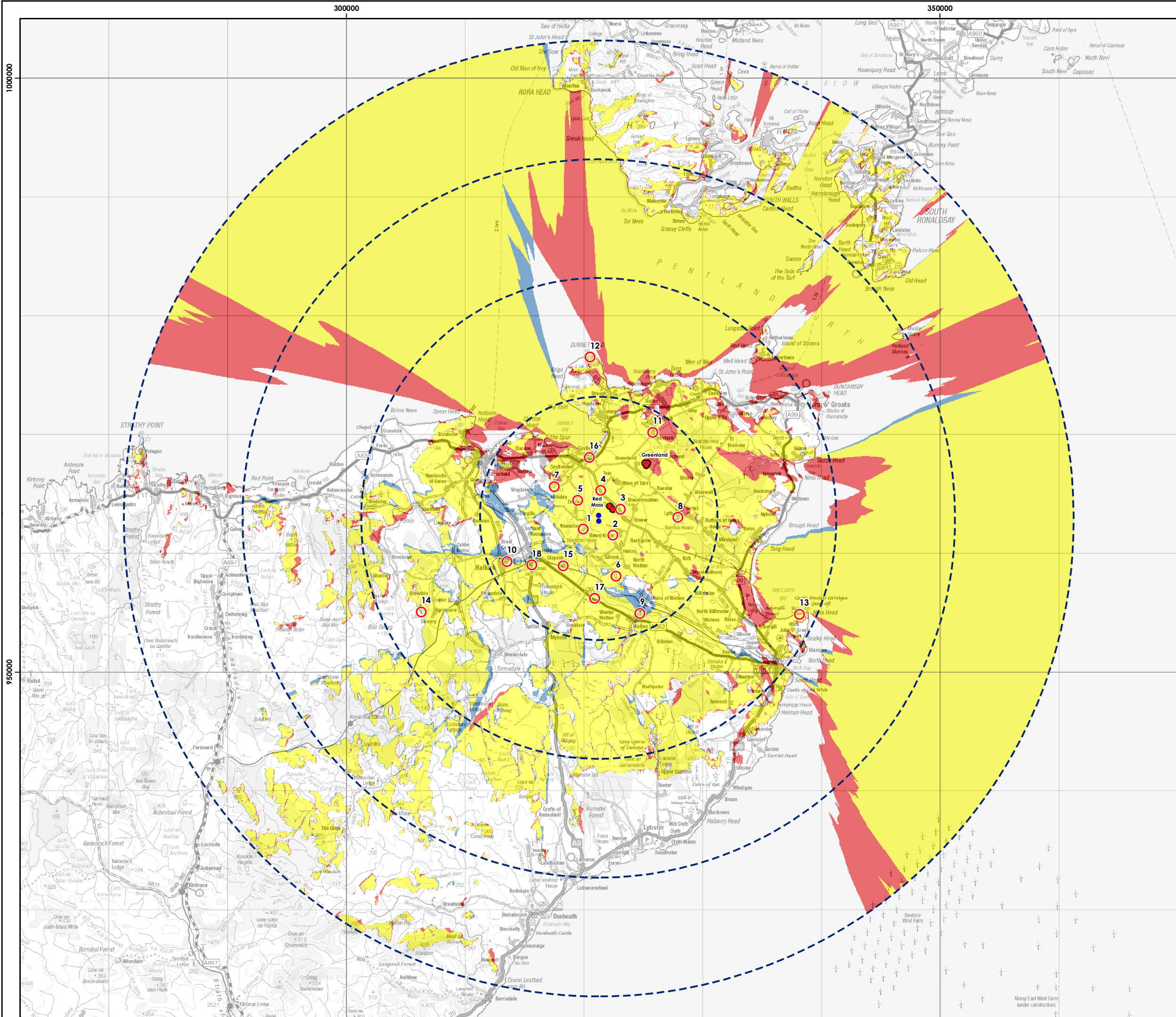
Figure 5-1-9c Cumulative Blade Tip ZTV: Greenland and Red Moss
