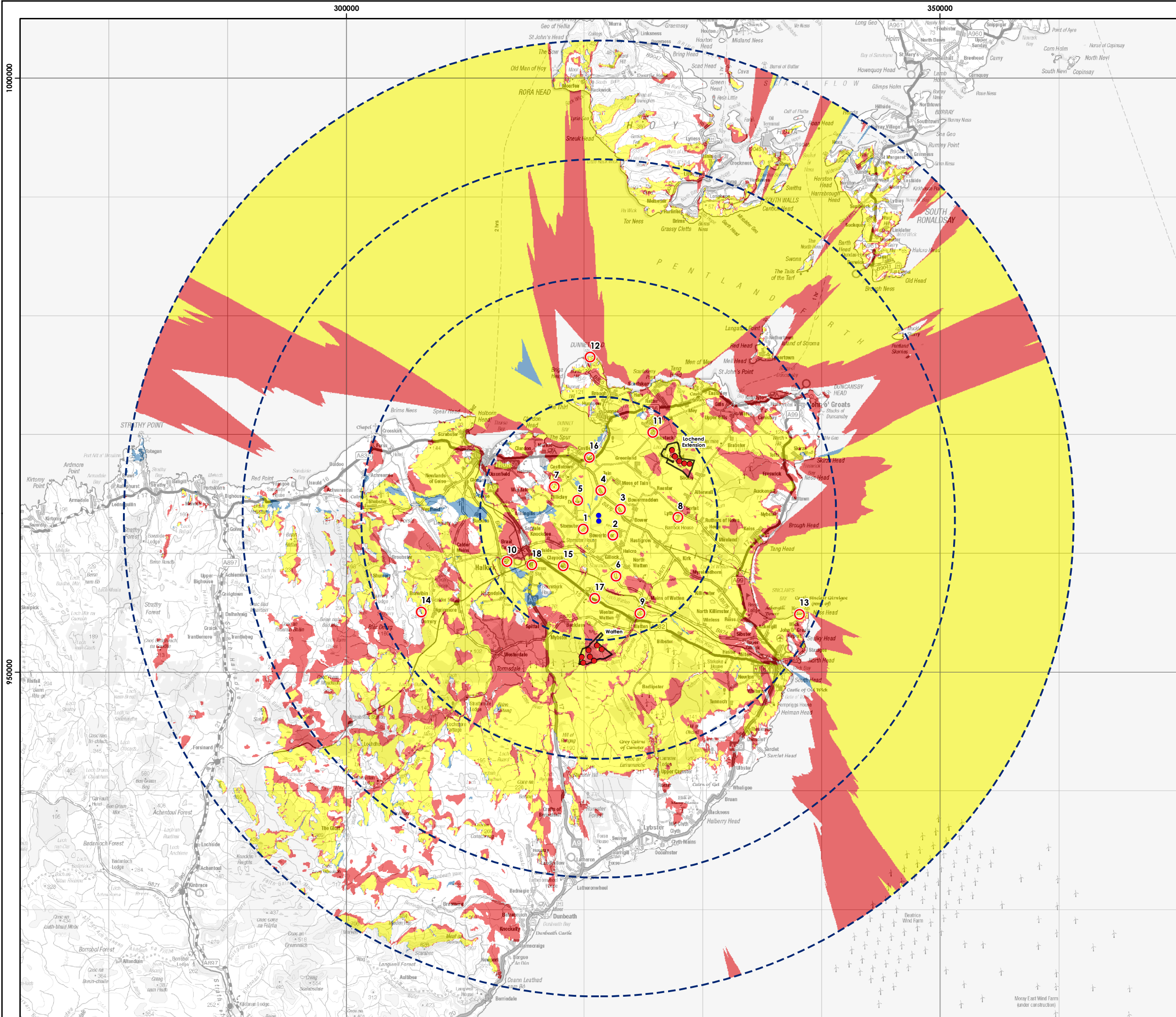
Figure 5-1-9d Cumulative Blade Tip ZTV: Lochend Extension & Watten
